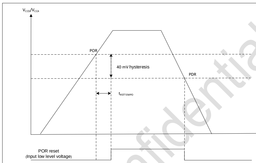
Figure 2-3 POR/PDR thresholds
