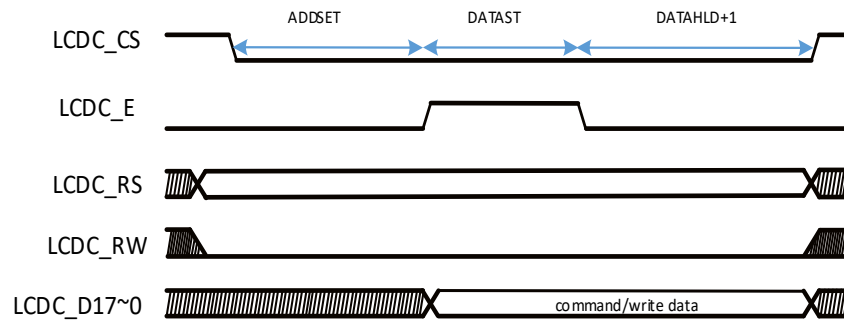
Figure 5-16 6800 mode write timing
