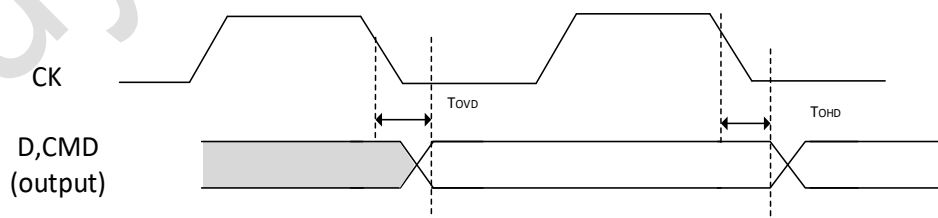
Figure 5-19 SDIO default mode
