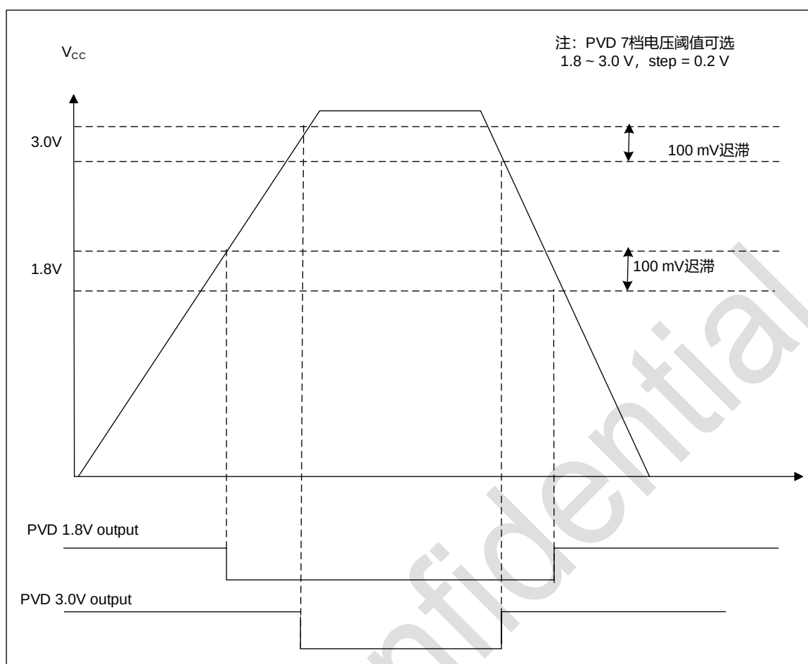
Figure 2-4 PVD threshold
