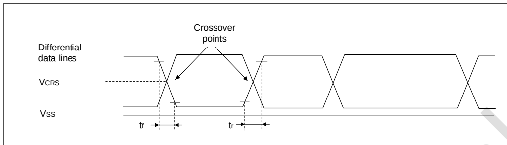
Figure 5-10 USB timing: data signal rise and fall time definition
