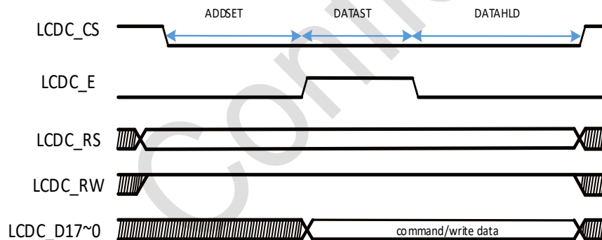
Figure 5-17 6800 mode read timing figure
