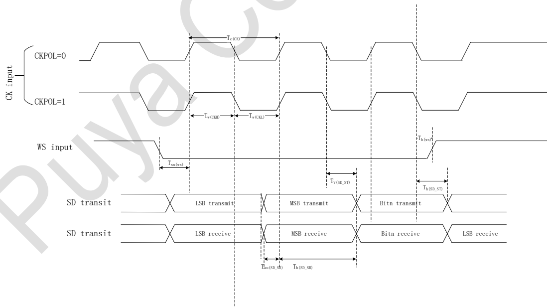
Figure 5-8 I 2 S slave timing diagram (Philips protocol)
