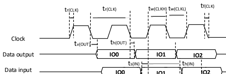
Figure 5-20 ESMC timing diagram-SDR Mode
