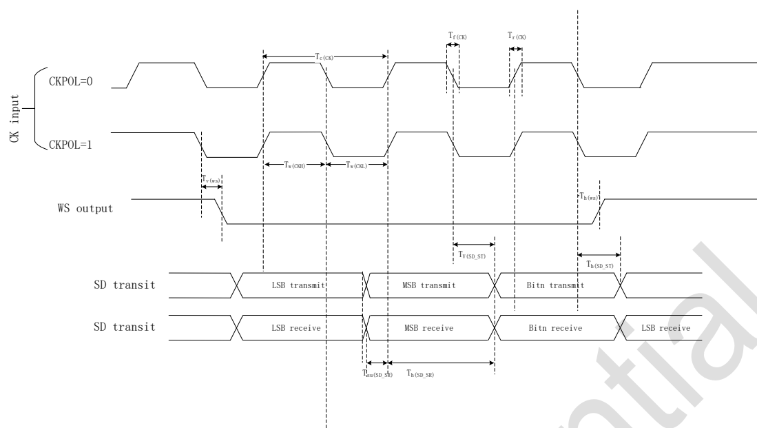
Figure 5-9 I²S master timing diagram (Philips protocol)
