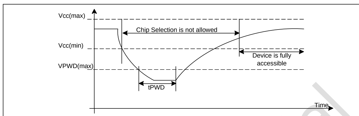
Figure 5-1 Power-on / power-down timing
