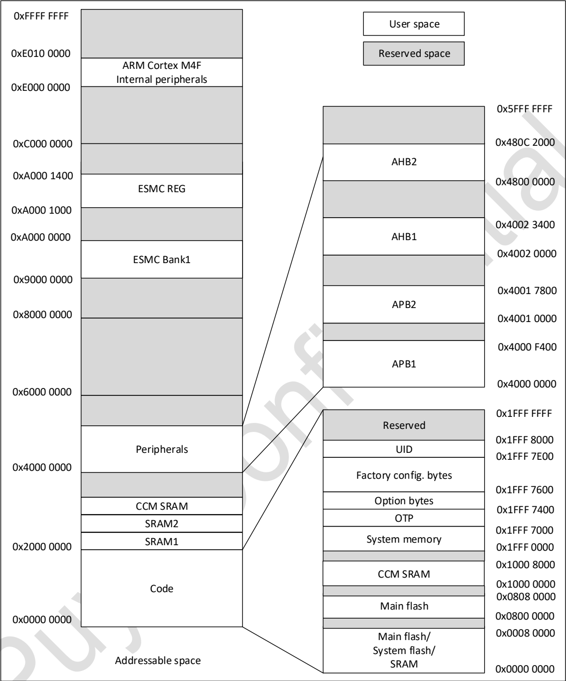
Figure 4-1 Memory mapping
