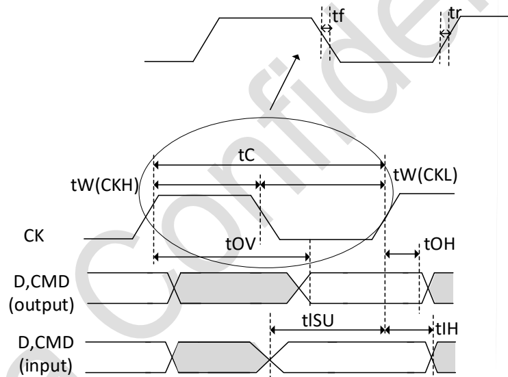
Figure 5-18 SDIO high-speed mode
