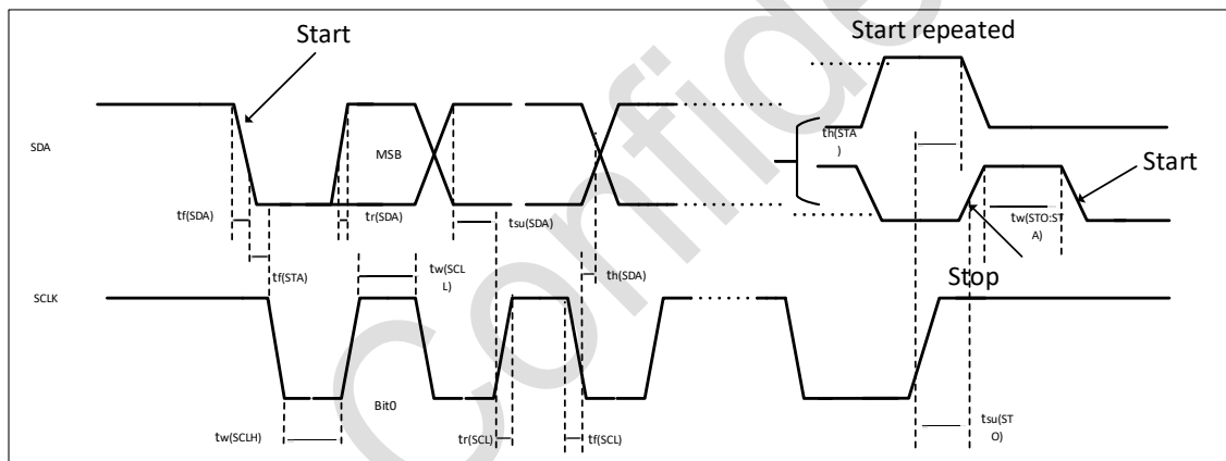
Figure 5-4 I 2 C bus timing diagram
