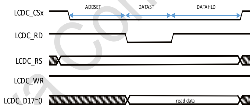
Figure 5-15 8080 Mode Read Timing Figure
