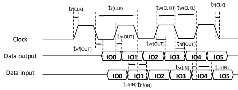
Figure 5-21 ESMC timing diagram-DDR Mode
