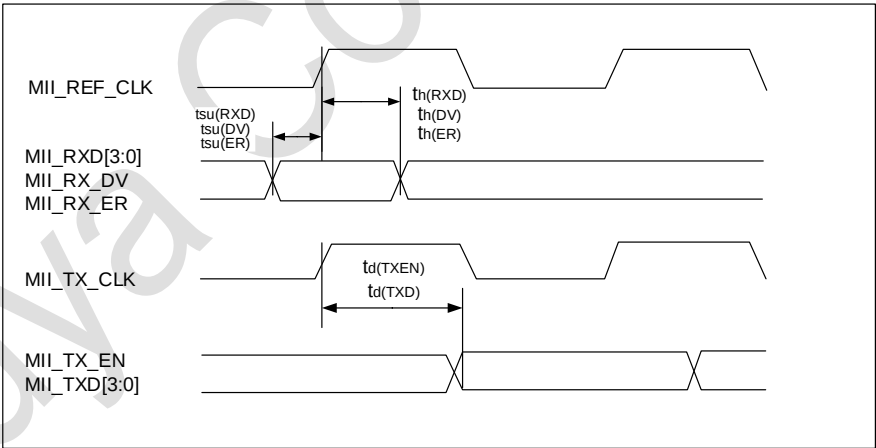
Figure 5-13 MII timing figure
