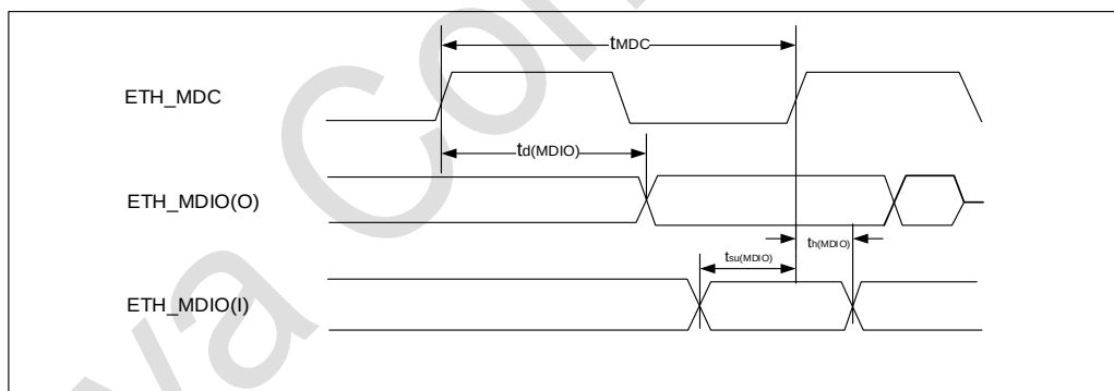
Figure 5-11 SMI timing figure
