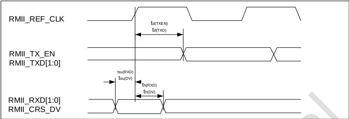
Figure 5-12 RMII timing
