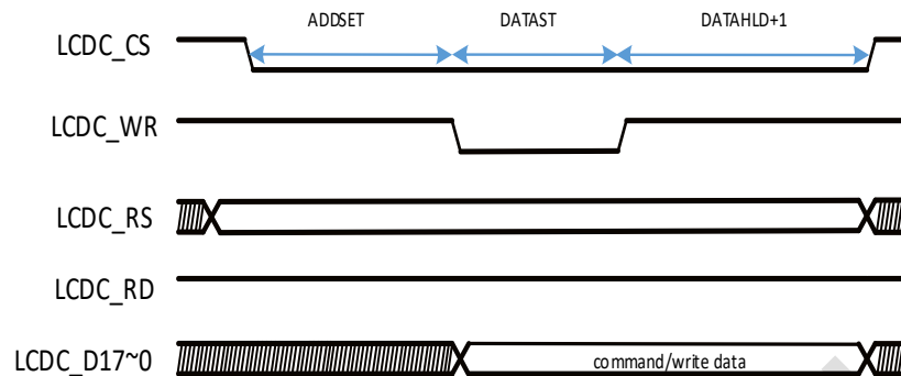
Figure 5-14 8080 mode write timing figure
