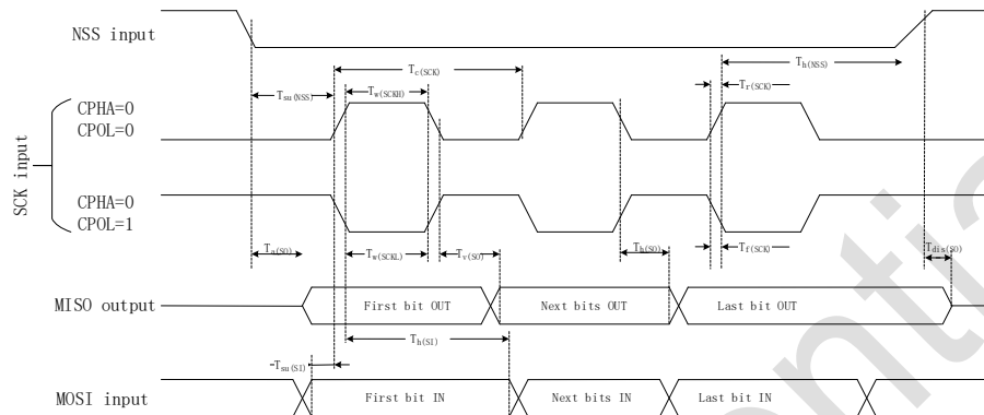
Figure 5-5 SPI timing diagram – slave mode and CPHA=0
